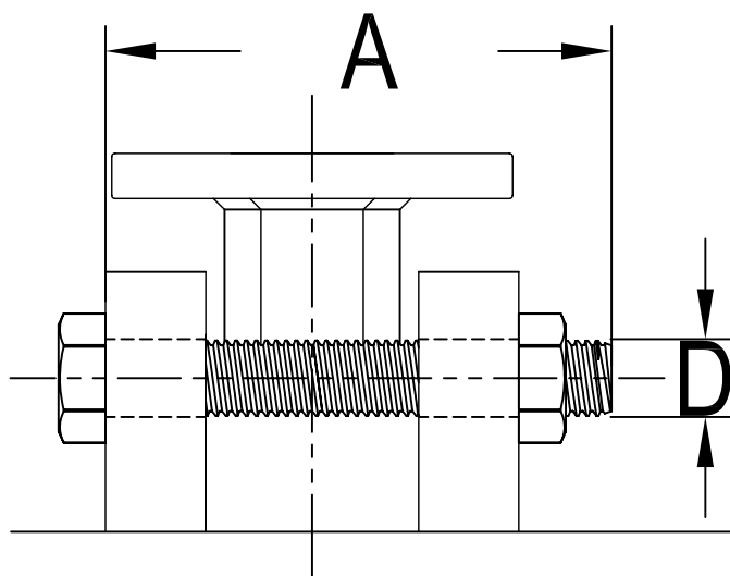
WAFER TYPE BUTTERFLY VALVE USING CROSS BOLTING
