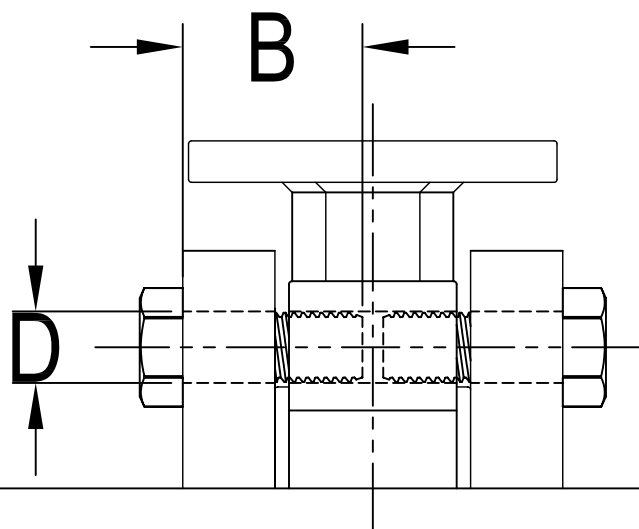
FULL LUG TYPE BUTTERFLY VALVE WITH TAPPED HOLES
